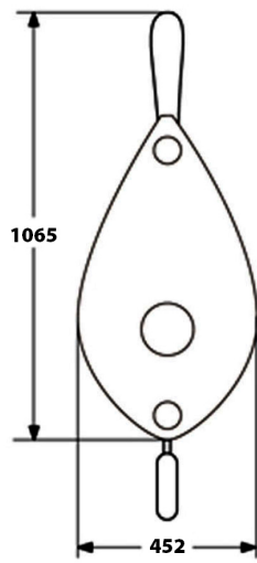
Wire Rope Ø=31 ~ 35
